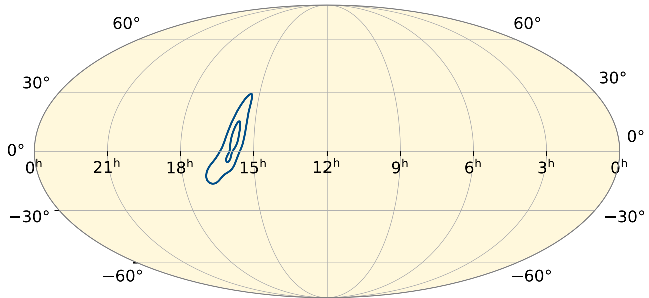
BAYESTAR
