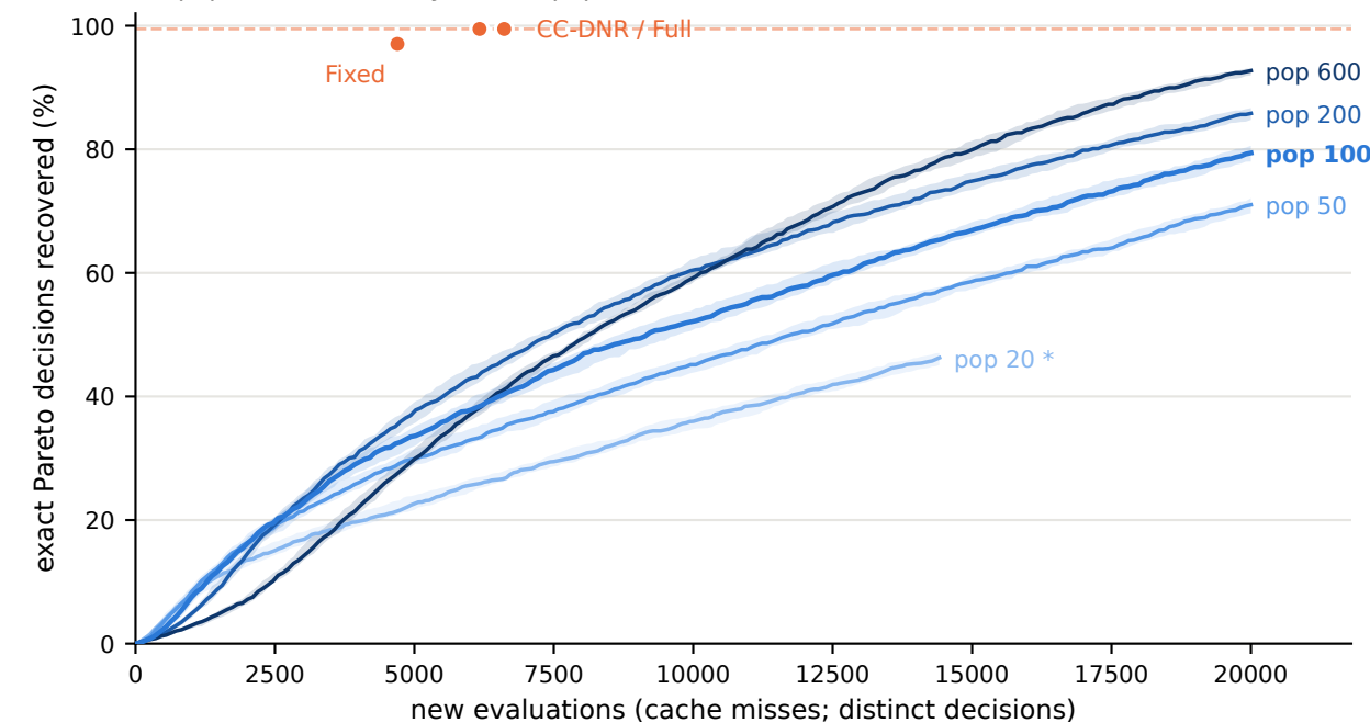
(a) population sensitivity; bold = pop 100 baseline
