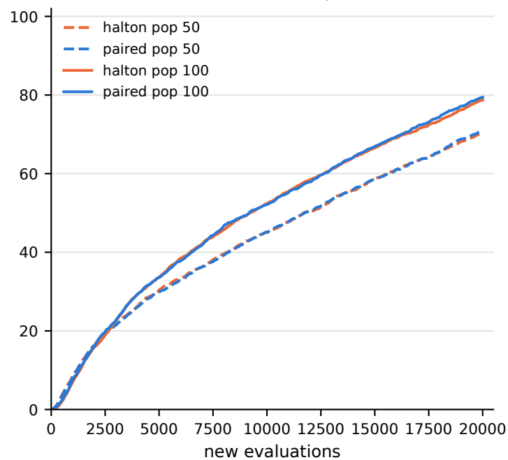
(b) initialization control: Halton vs paired random
