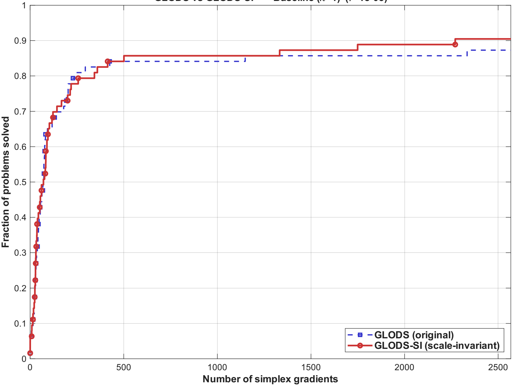
GLODS vs GLODS-SI — Baseline ( \kappa=1 ) ( \tau=1e-05 )
