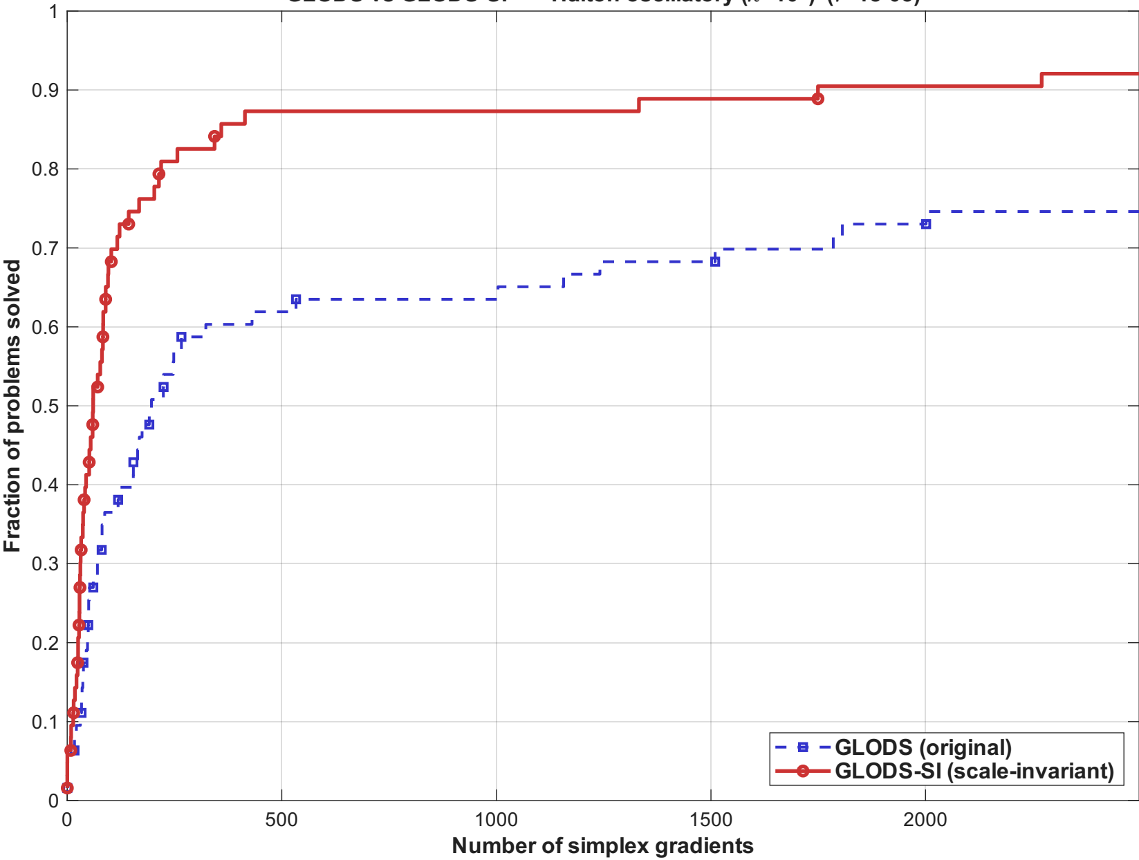
GLODS vs GLODS-SI — Halton oscillatory ( \kappa=10^6 ) ( \tau=1e-05 )
