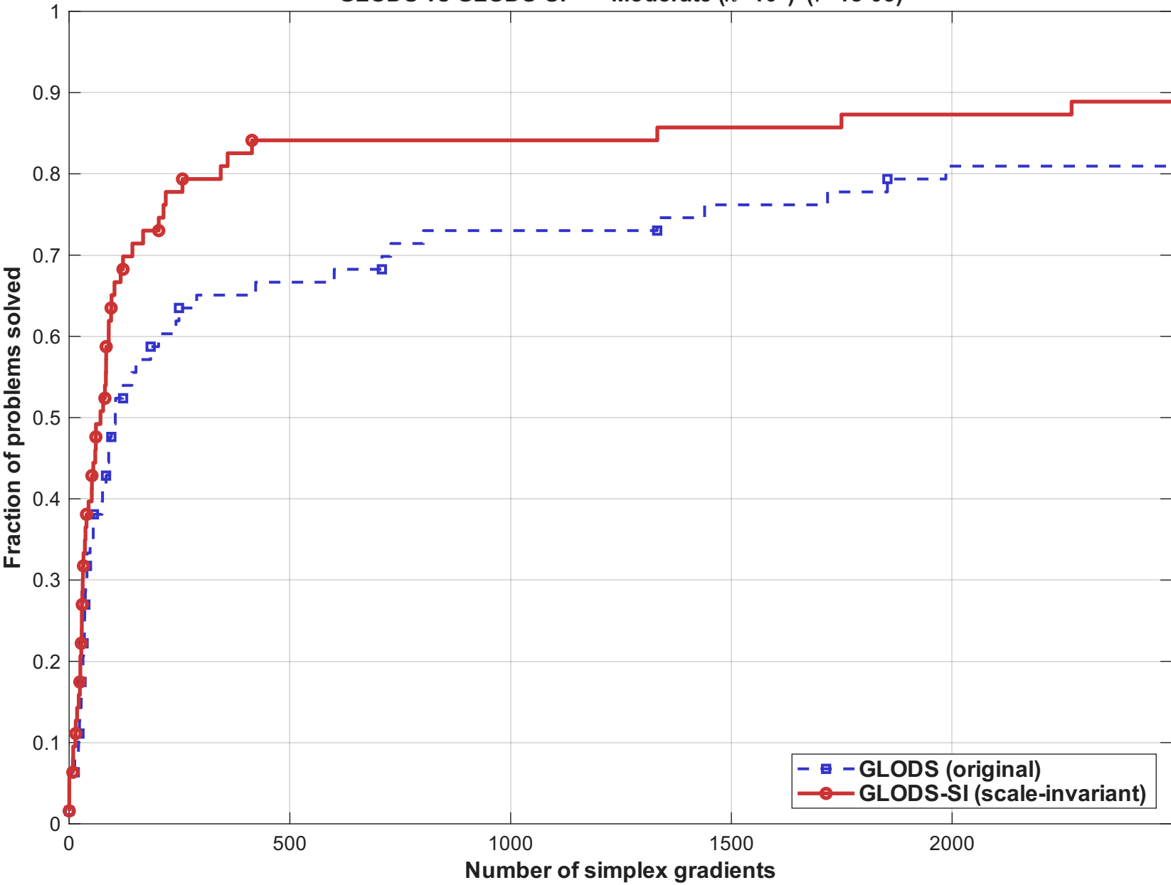
GLODS vs GLODS-SI — Moderate ( \kappa=10^4 ) ( \tau=1e-05 )
