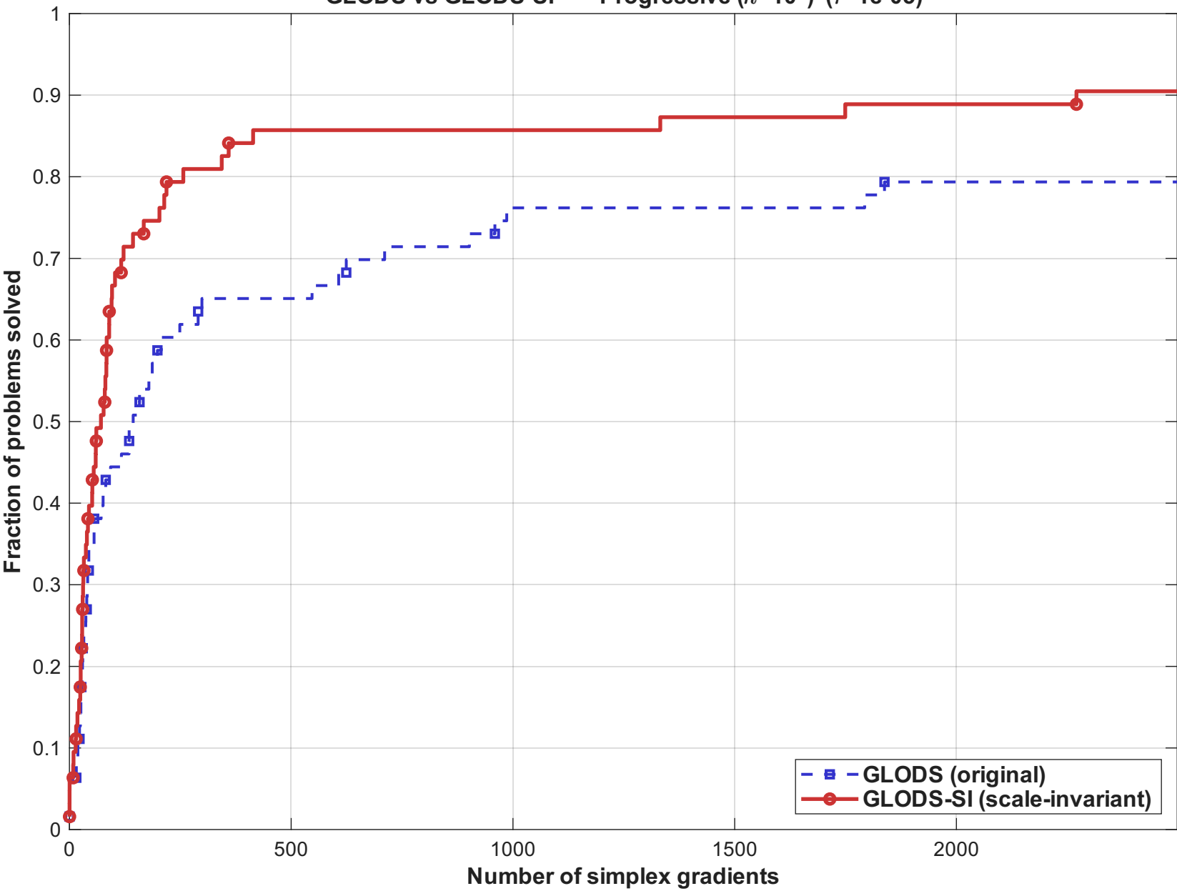
GLODS vs GLODS-SI — Progressive ( \kappa=10^6 ) ( \tau=1e-05 )
