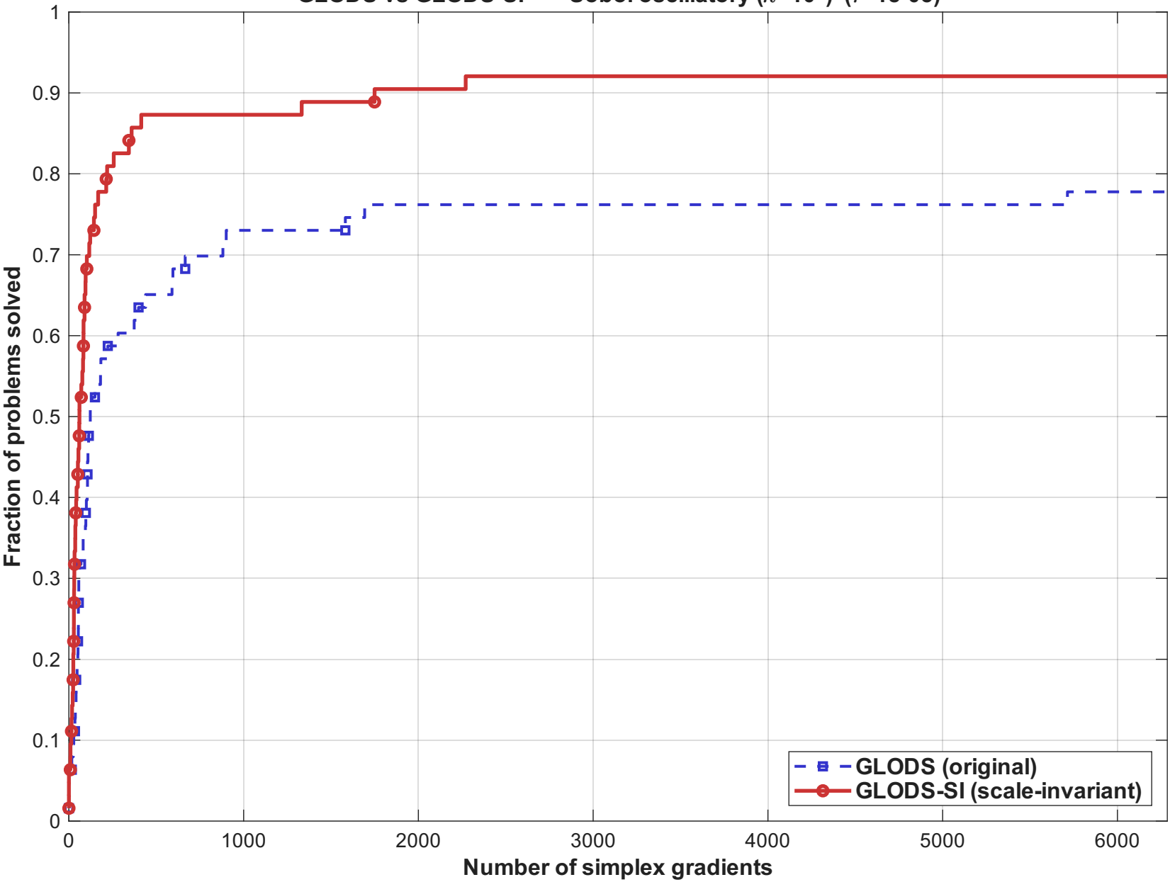
GLODS vs GLODS-SI — Sobol oscillatory ( \kappa=10^6 ) ( \tau=1e-05 )
