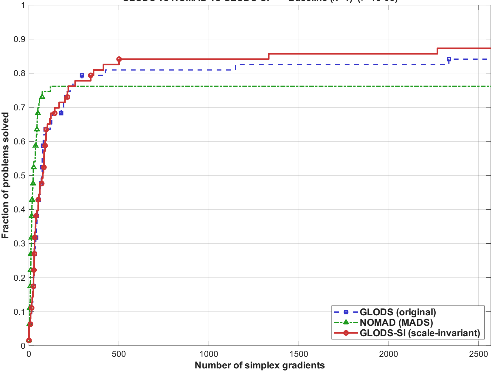
GLODS vs NOMAD vs GLODS-SI — Baseline ( \kappa=1 ) ( \tau=1\text{e-}05 )
