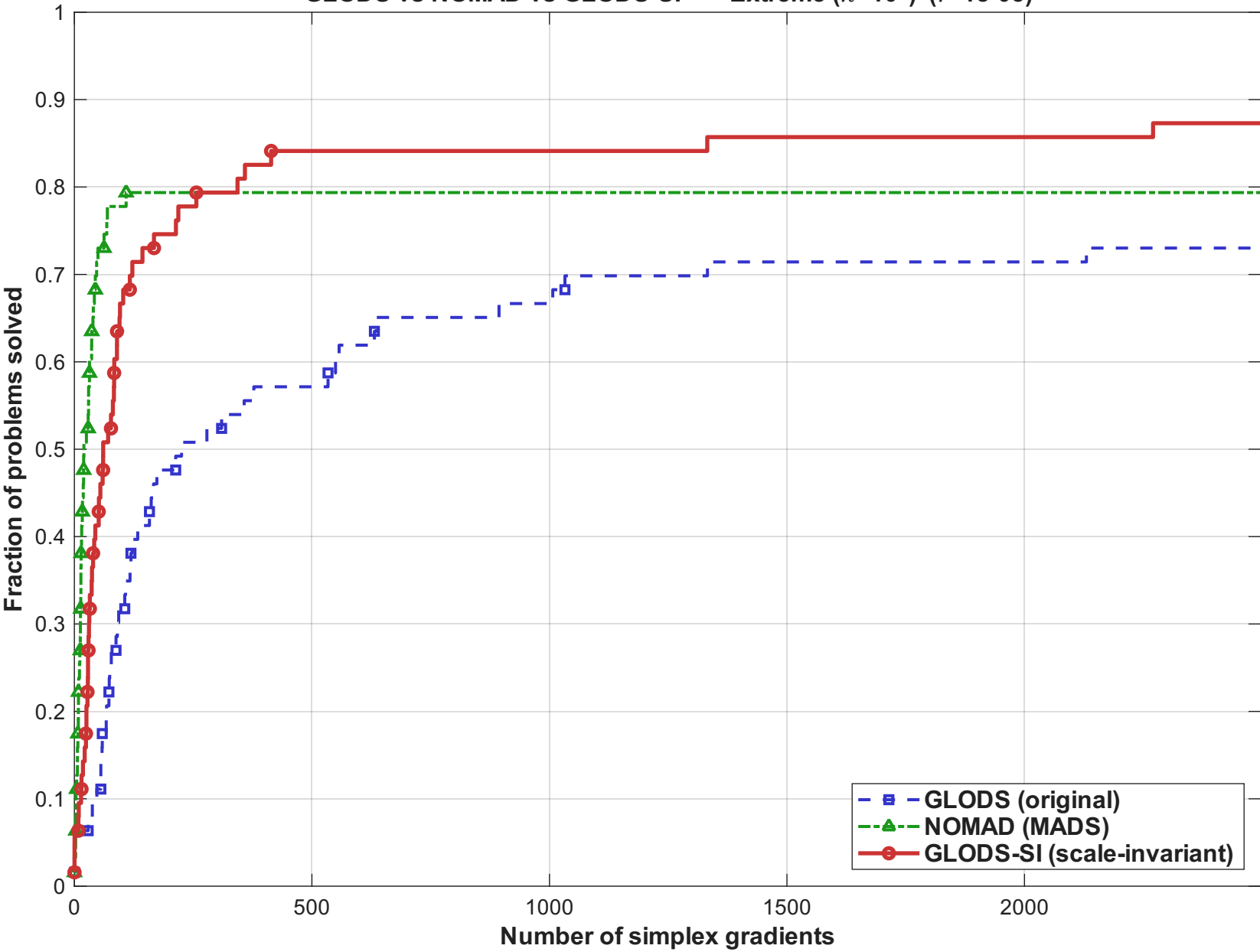
GLODS vs NOMAD vs GLODS-SI — Extreme ( \kappa=10^8 ) ( \tau=1e-05 )
