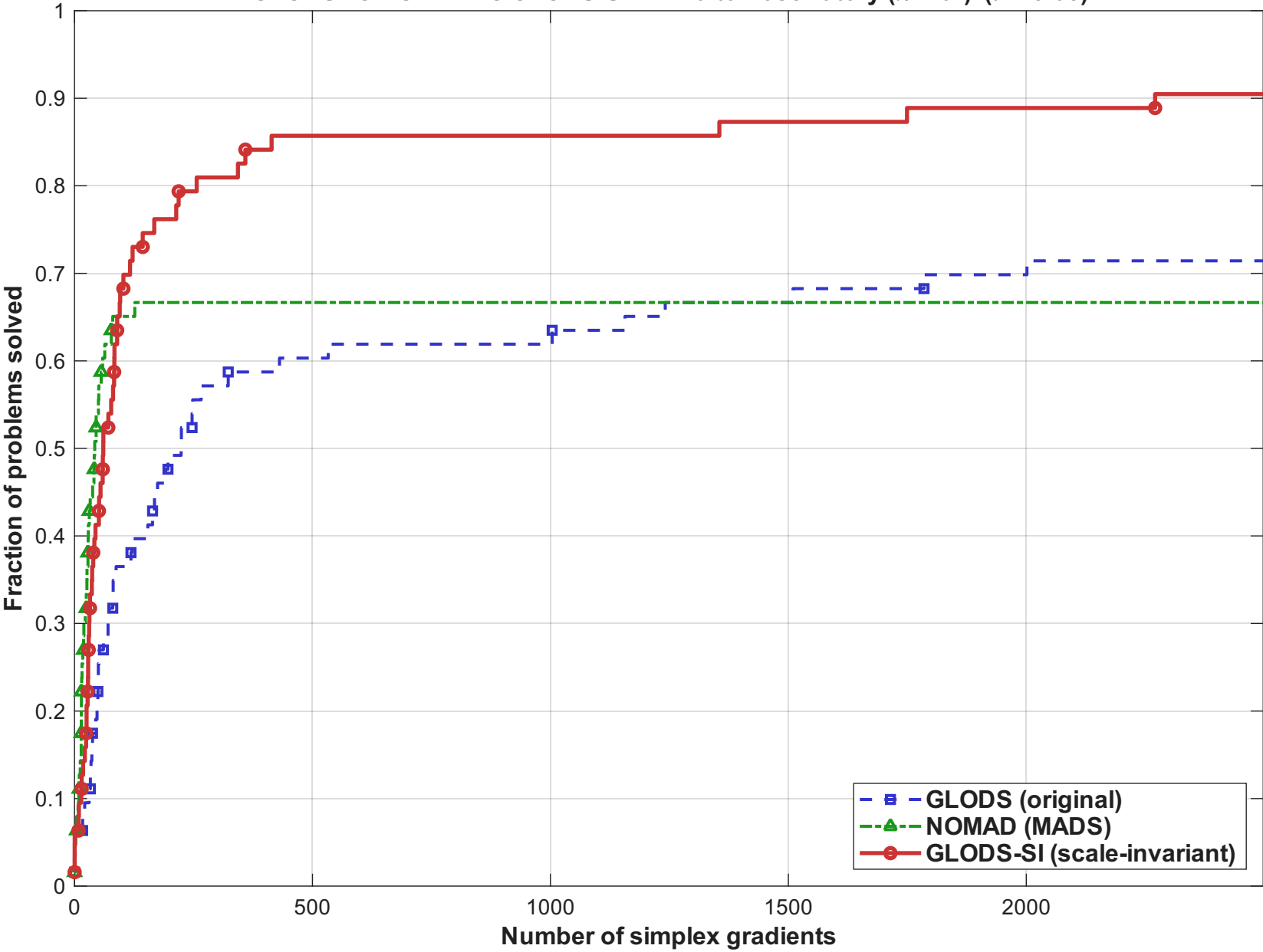
GLODS vs NOMAD vs GLODS-SI — Halton oscillatory ( \kappa=10^6 ) ( \tau=1e-05 )
