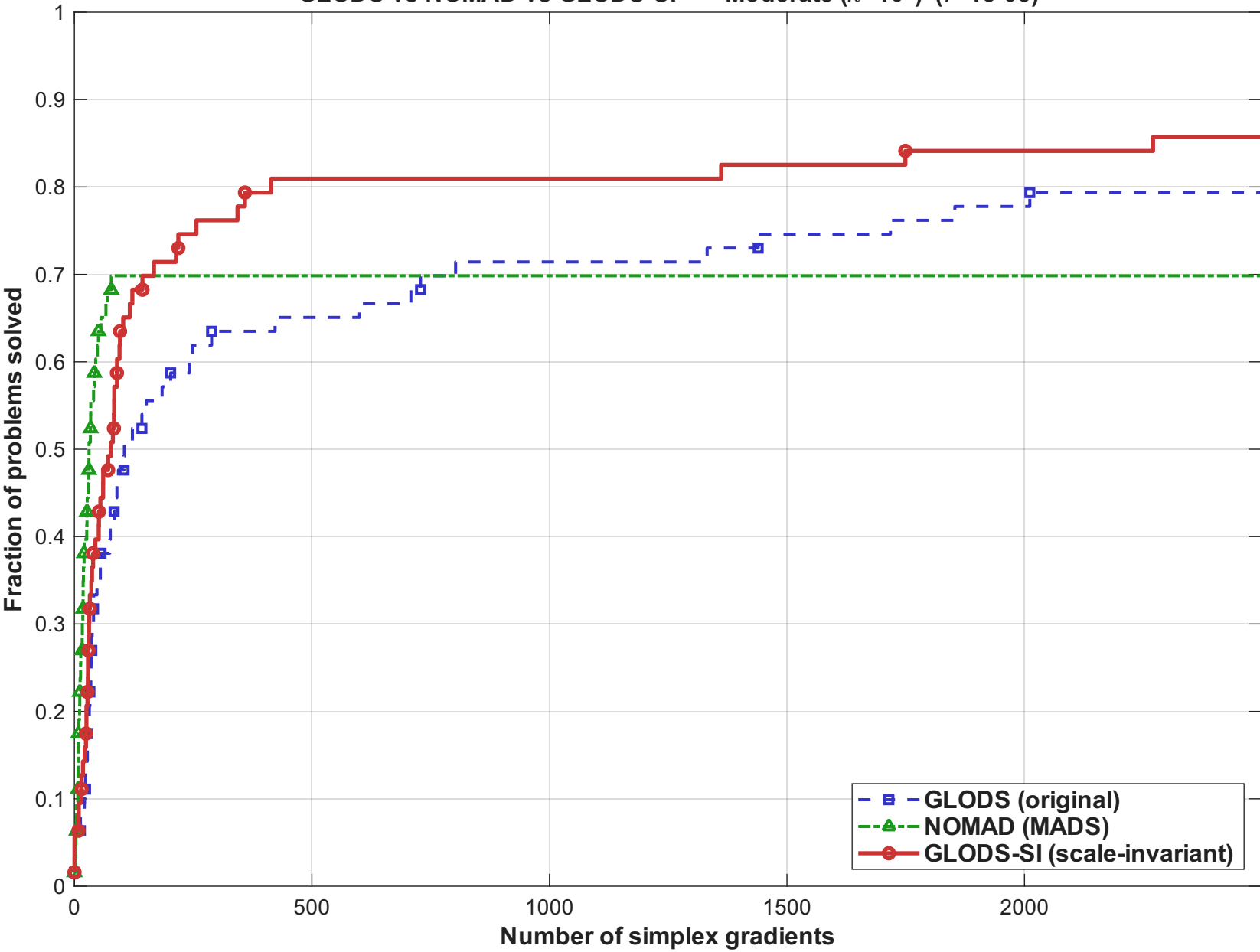
GLODS vs NOMAD vs GLODS-SI — Moderate ( \kappa=10^4 ) ( \tau=1e-05 )
