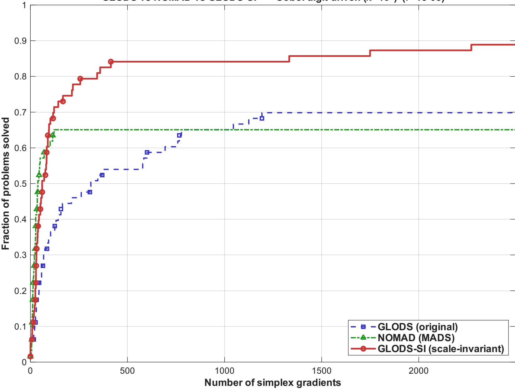
GLODS vs NOMAD vs GLODS-SI — Sobol digit-driven ( \kappa=10^8 ) ( \tau=1e-05 )
