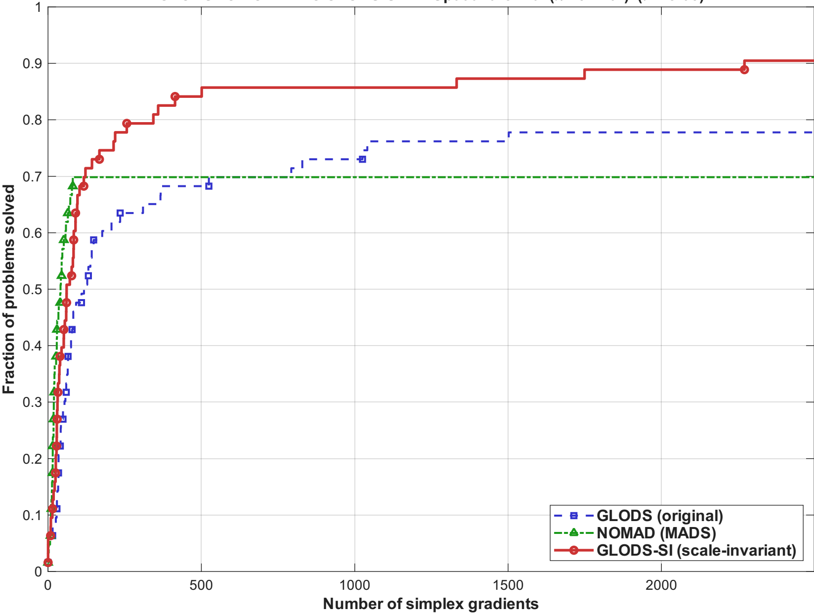
GLODS vs NOMAD vs GLODS-SI — Spatial-thermal ( \kappa \approx 9 \times 10^4 ) ( \tau = 1e-05 )
