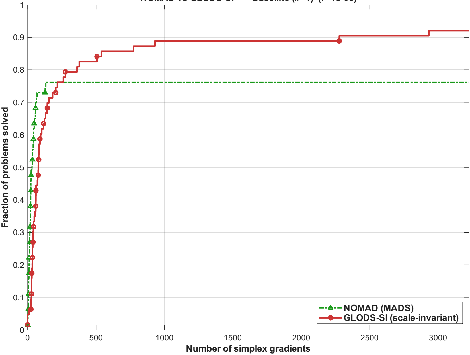
NOMAD vs GLODS-SI — Baseline ( \kappa=1 ) ( \tau=1e-05 )
