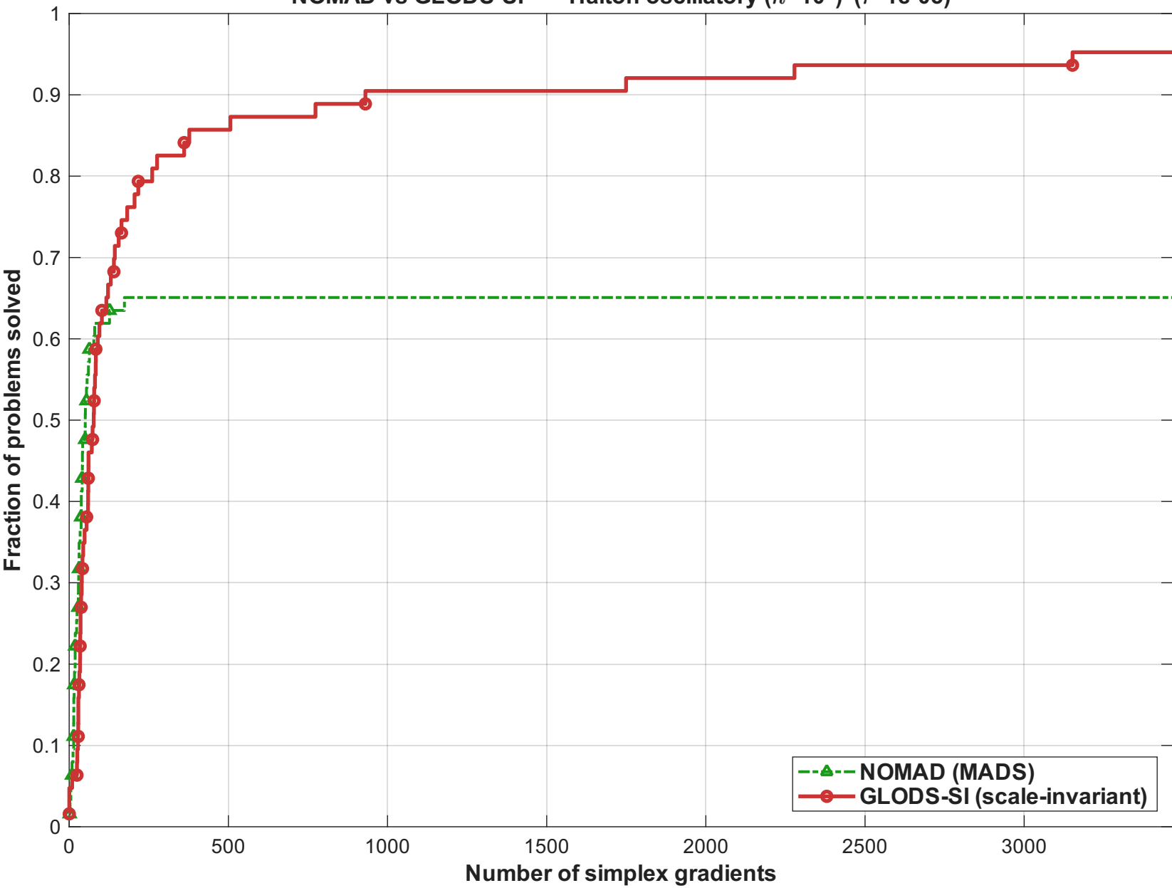
NOMAD vs GLODS-SI — Halton oscillatory ( \kappa=10^6 ) ( \tau=1e-05 )
