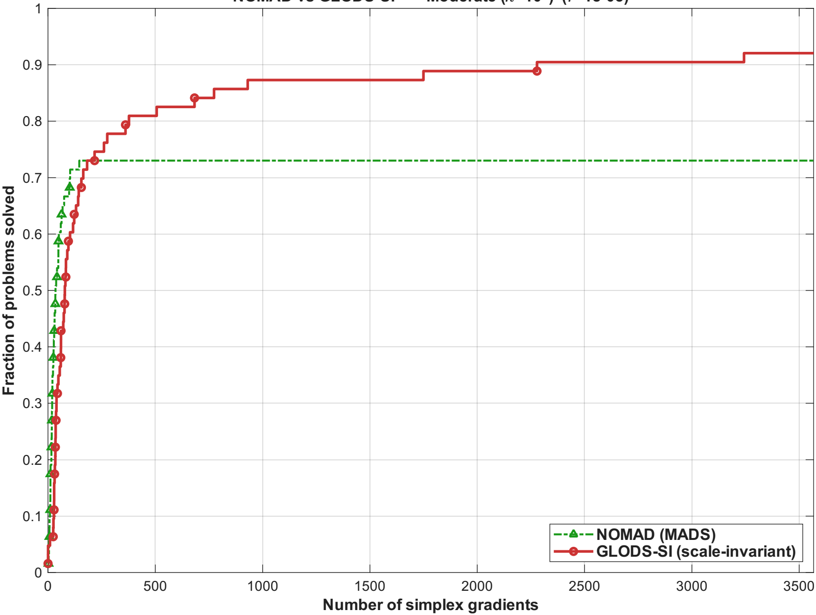
NOMAD vs GLODS-SI — Moderate ( \kappa=10^4 ) ( \tau=1\text{e-}05 )
