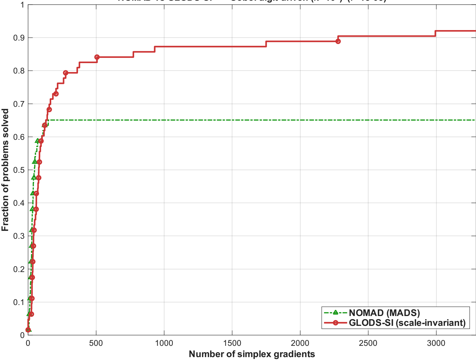
NOMAD vs GLODS-SI — Sobol digit-driven ( \kappa=10^8 ) ( \tau=1e-05 )
