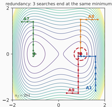
Aluffi-Pentini on [-2, 2]^2 (the sequence from the 2015 presentation, redone).
