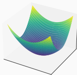
unimodal: f = 0,5x_1^2 + x_2^2
