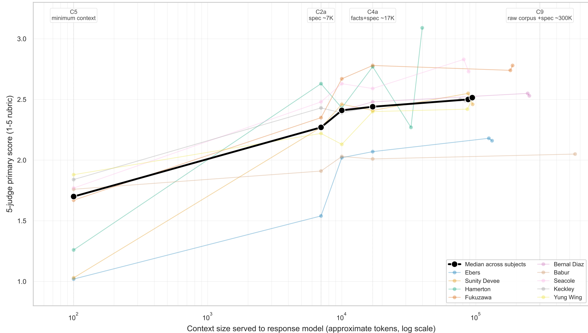
Figure 4.2 — Compression: score vs. context size across low-baseline subjects
