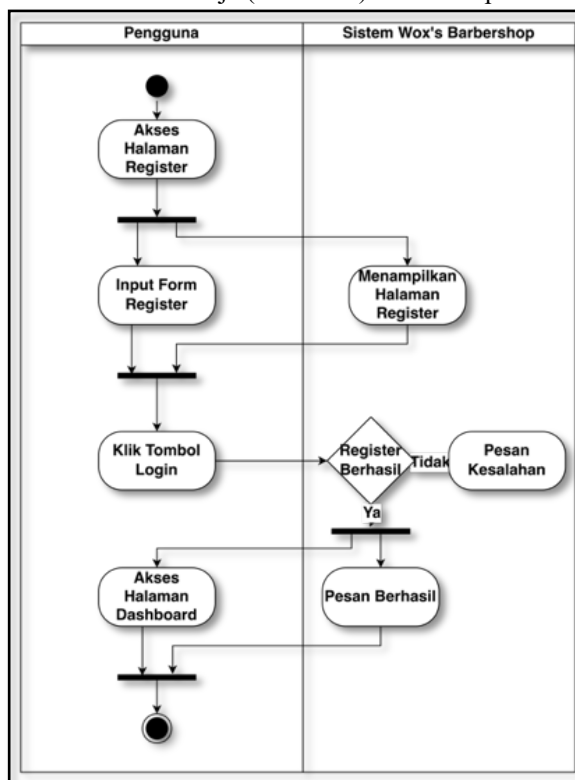
Gambar 3. Activity Diagram
