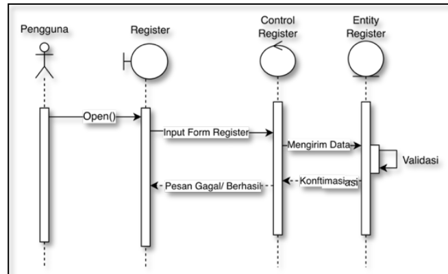
Gambar 3. Sequence Diagram
