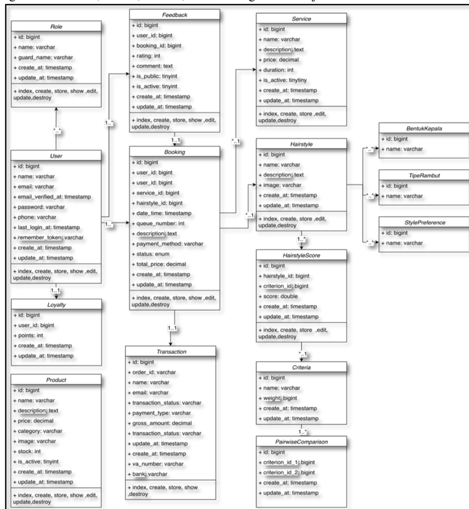
Gambar 3. Class Diagram
