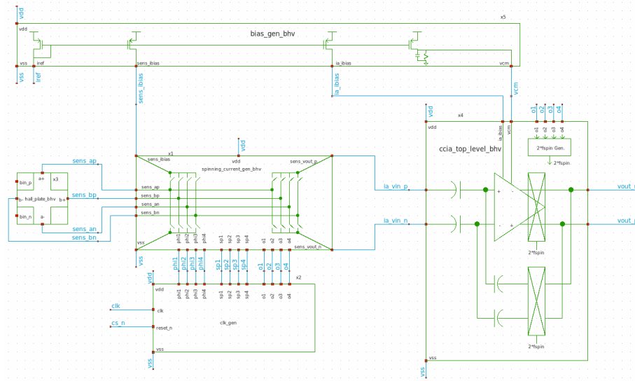
Figure 2: More detailed block diagram of top level schematic, showing the detailed connection between all blocks, excluding the SPI configuration interface. The Hall plate (left) is connected to the spinning current generator (center), which periodically swaps the bias/readout terminals of the sensor prior to amplification and demodulation by the instrumentation amplifier (right). The internal clocks are generated by the clock generator block (bottom) and all bias currents are derived from an external reference in the bias generator block (top).
