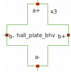
Figure 3: Xschem schematic symbol for on-chip Hall plate, showing (a+, b+, a-, b-) pin orientation and naming convention.
