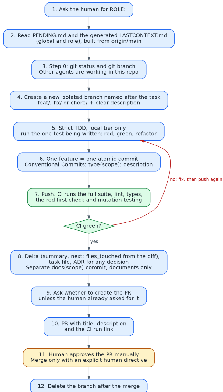
Figure 2. The life of a task, from asking for a role to deleting the branch after the merge.
