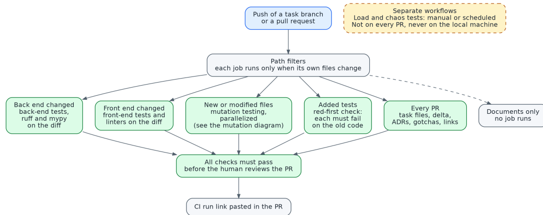
Figure 4. The CI pipeline. Path filters route a change to parallel jobs, including the red-first check; load and chaos tests are separate workflows.
