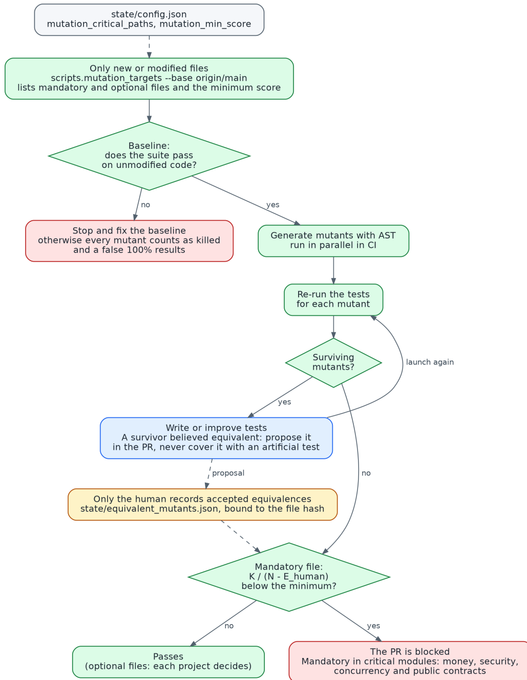
Figure 5. Mutation testing on the diff, with the baseline check, human-only acceptance of equivalent mutants, and the blocking rule for mandatory files.
