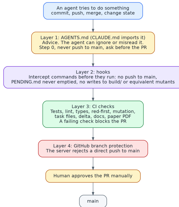
Figure 6. Control layers. The layers are shown in a rough order; in practice each acts at a different moment.
