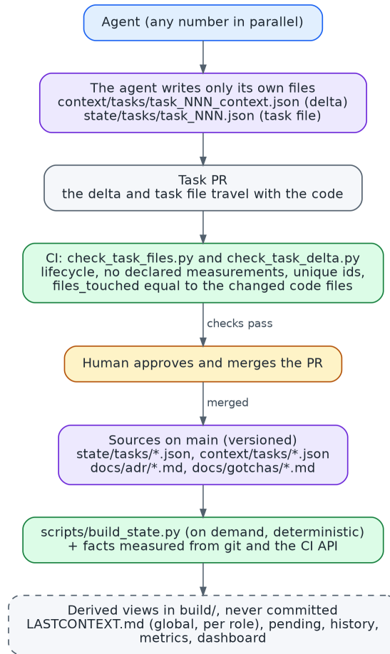
Figure 3. State and context. The agent writes only its own delta and task file; CI checks the delta against the diff; the shared views are derived from origin/main on demand and never committed.
