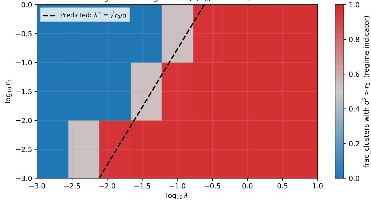
Phase diagram: V7 regime vs (\lambda, r_0) at d=17, 30 seeds
