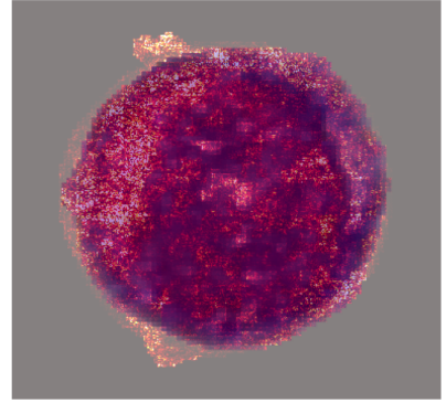
SHAP Overlay
