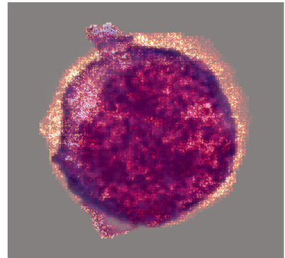
SHAP Overlay
