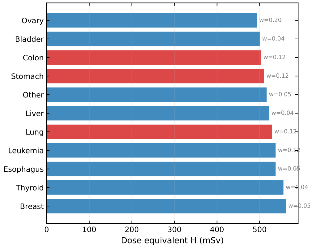
Organ Dose Equivalent — 16 g/cm² Al (259-day transit)
