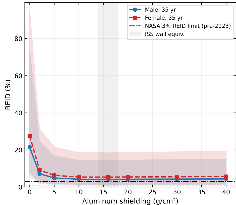
REID vs Shielding — 259-day Transit (launch 2031-01-01)
