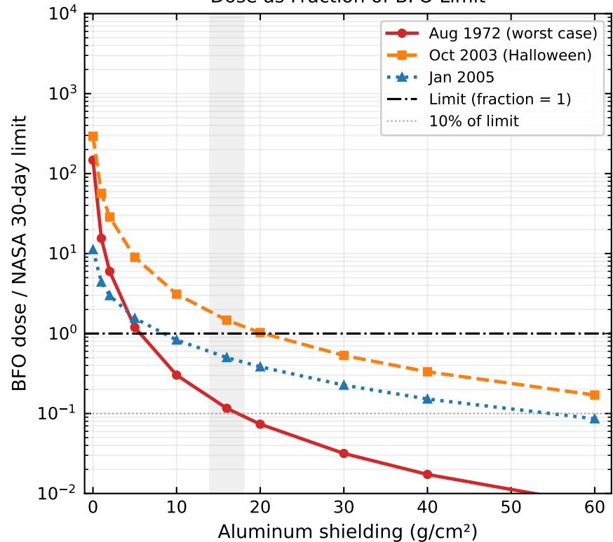
Dose as Fraction of BFO Limit
