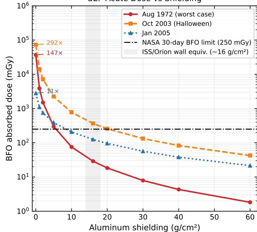
SEP Acute Dose vs Shielding
