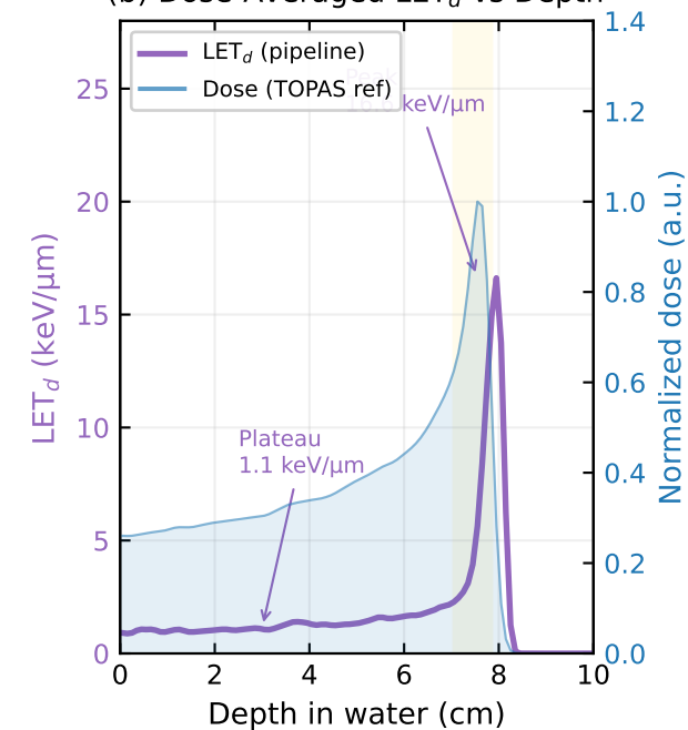
(b) Dose-Averaged LET_d vs Depth
