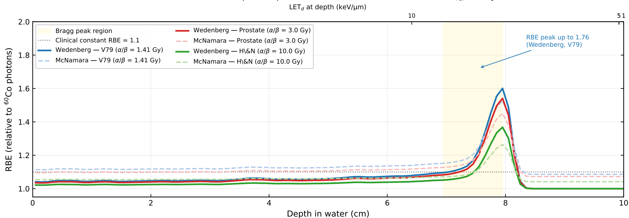
(c) Proton RBE vs Depth — Pipeline vs Clinical Models (100 MeV beam, D_{ref} = 4 Gy)
