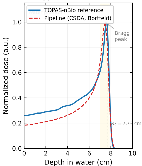
(a) Bragg Curve — 100 MeV Proton
