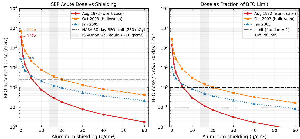
Figure 3: SEP acute BFO dose vs. aluminum shielding. Left: absolute dose (mGy); horizontal line = NASA 30-day BFO limit (250 mGy); shaded band = ISS/Orion wall equivalent ( 14\text{--}18\text{ g cm}^{-2} ). Multiples of the limit are annotated at zero shielding. Right: same data normalized to the BFO limit.
