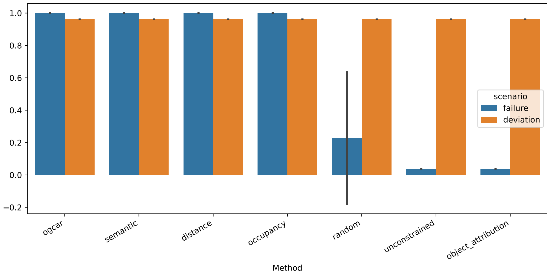
Deviation Reduction@k
