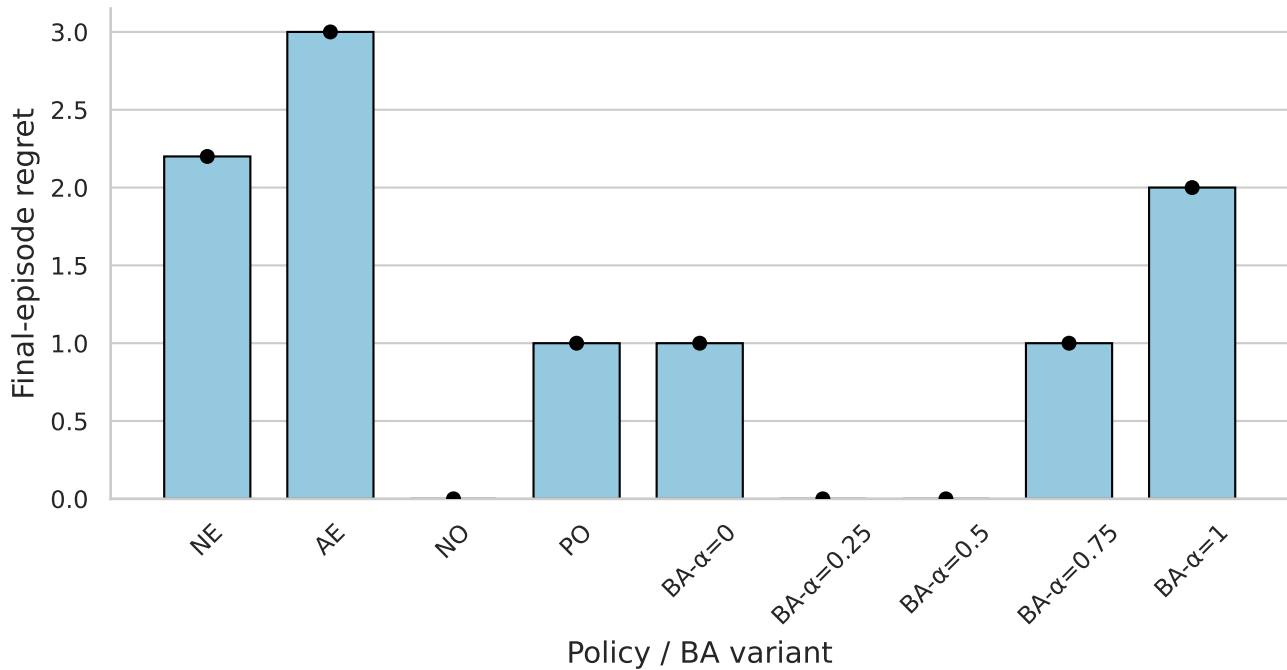
Experiment 1: final-episode regret per variant
