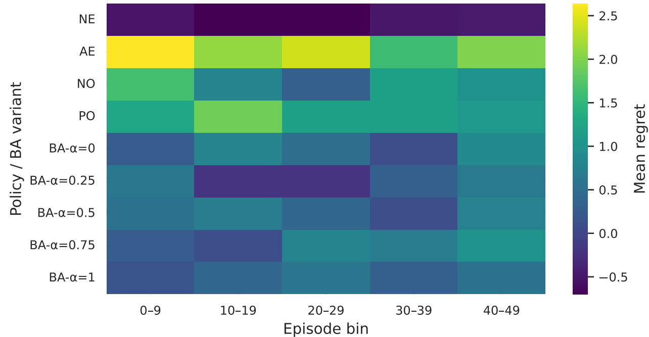
Experiment 1: regret over time (binned heatmap)
