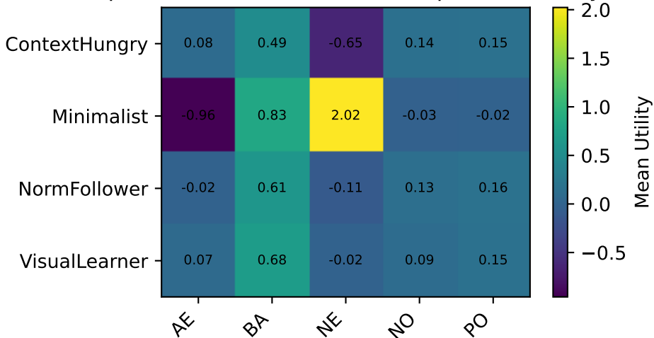
Experiment 2: Fairness Heatmap (Mean Utility)
