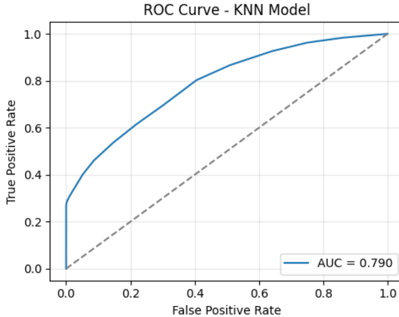
Figure 4: ROC Curve for the KNN Model
