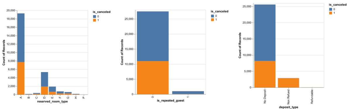
Figure 2: EDA bar plots: Reserved Room Type, Repeated Guest Status, and Deposit Type vs Cancellations.
