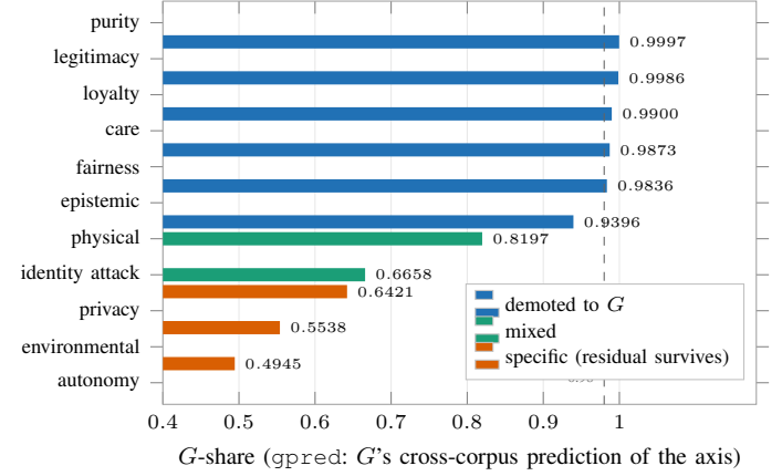
Fig. 3. Bifactor readout (Phase A2). Five axes sit at or above 0.98 G -share (dashed line): their gate-passing transfer is general valence, not their named dimension, and the standing specificity gate demotes them (colors follow the gate verdict; the gate additionally demotes epistemic and adjudicates identity_attack specific—the one divergence between the methods, recorded in the text). Privacy, environmental, and autonomy carry genuinely axis-specific signal.
