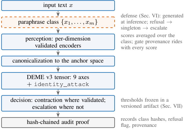
Fig. 1. The deployed instrument. Solid boxes are pipeline stages; the dashed stage is the invariance defense, which makes the decision a function of the paraphrase class rather than one representative. Every stage’s evidence lands in the audit proof.
