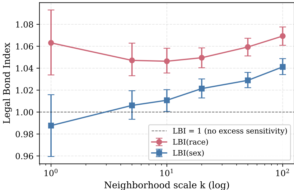
COMPAS LBI by protected attribute, across neighborhood scales
