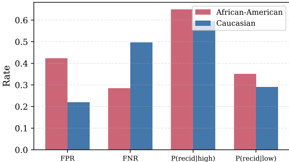
Standard fairness metrics: COMPAS by race
