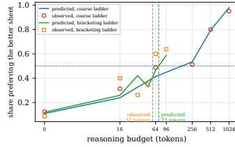
Figure 3: Where the preference turns over. The share of test pairs on which the judge prefers the better worksheet, against the reasoning budget it was allowed. Lines are predicted from calibration blocks, points are sealed test blocks, on the first ladder and on the second, which brackets the crossing. On the first the crossing was predicted at 174 tokens and observed at 128, 0.37 noise units against a bar of 2.576. On the second it was predicted at 72 and observed at 57, 0.62 noise units, and the spread of the comparison fell from a factor of 2.2 to 1.4.
