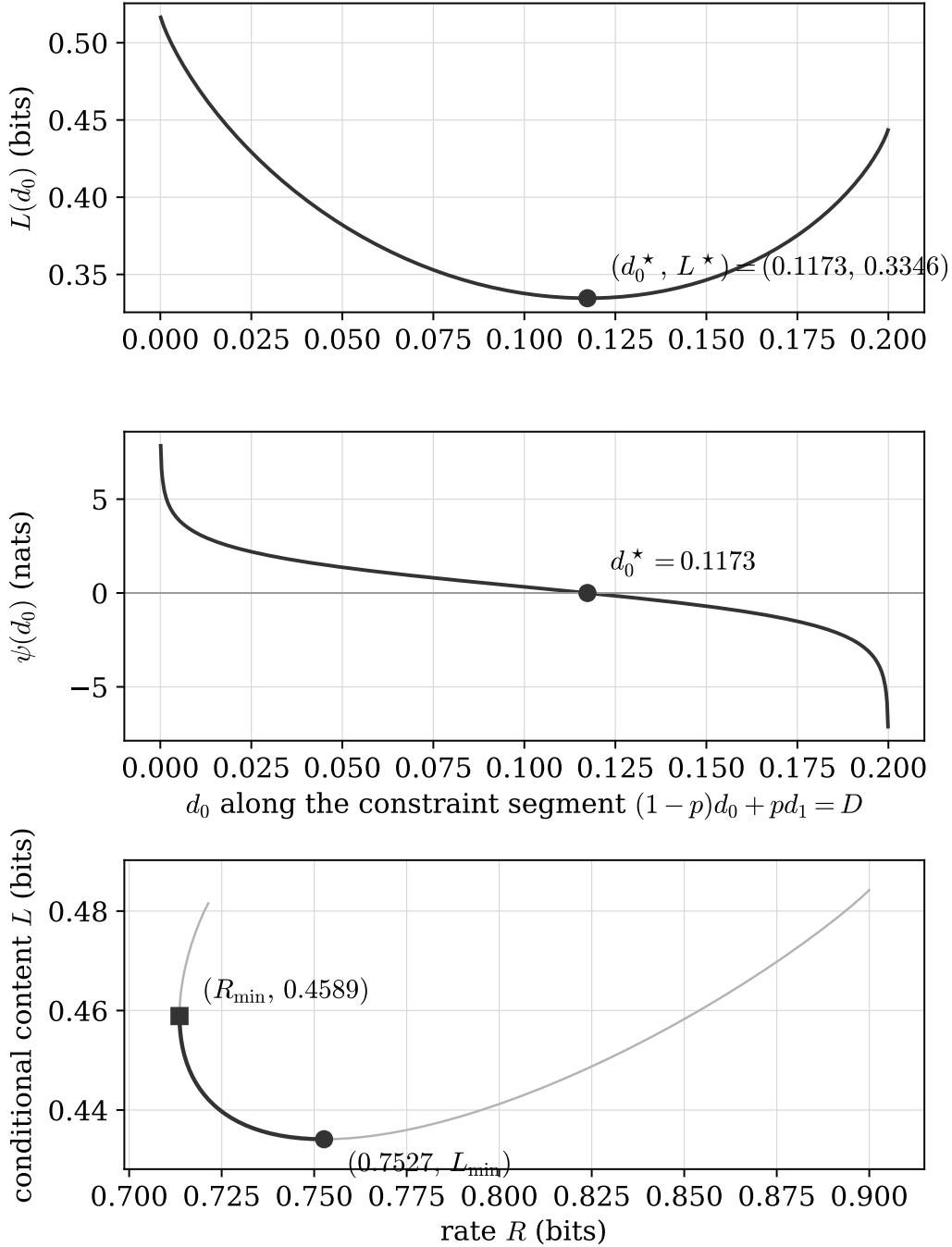
Fig. 5. The binary objective L(d_0) (top) and the tilt residual \psi(d_0) (middle) along the constraint segment (1-p)d_0 + pd_1 = D at (p, q, D) = (0.25, 0.15, 0.15) : the residual crosses zero exactly once, at d_0^* = 0.1173 ( d_1^* = 0.2480 ), and L attains its unique minimum 0.3346 bits there, as Lemma 26 asserts. Bottom: the binary rate–content frontier at (p, q, D) = (0.1, 0.1, 0.05) , the curve (R(d_0), L(d_0)) along the segment (Remark 28), with the Pareto arc from the tilt root d_0^* = 0.0282 (the L -minimizer, L_{\min} = 0.4341 bits) to d_0 = D (the R -minimizer, R_{\min} = 1 - h_2(D) = 0.7136 bits) drawn bold. The tradeoff is strict: the L -optimal point pays 0.0391 bits of excess rate and the R -optimal point pays 0.0248 bits of excess conditional content.
