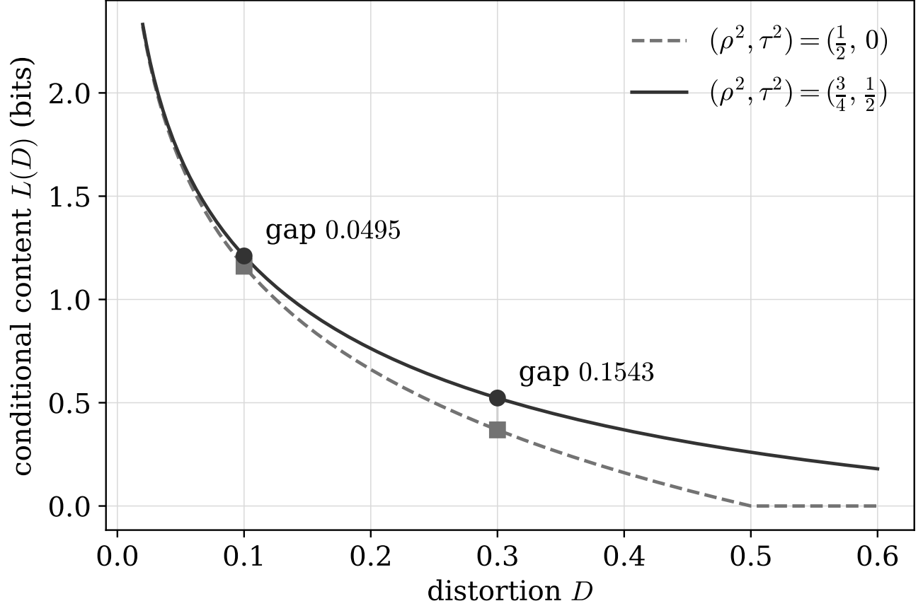
Fig. 4. Non-determination by the reduced marginal (Corollary 21): L(D) against D for the two instances (\rho^2, \tau^2) = (\frac{1}{2}, 0) (dashed, squares) and (\frac{3}{4}, \frac{1}{2}) (solid, circles), which share the reduced correlation \text{Corr}(Y, S) = \rho/\sqrt{s} = 1/\sqrt{2} = 0.7071 . The two functions differ at every distortion shown; at the tabulated levels (markers; Table III) the gap is 0.0495 bits at D = 0.1 and 0.1543 bits at D = 0.3 .
