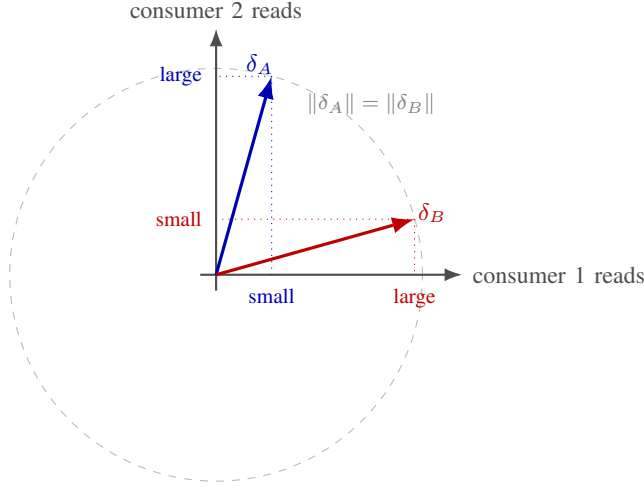
Fig. 1. The flip. Two lossy codes produce errors \delta_A, \delta_B of equal reconstruction norm (dashed circle), so reconstruction cannot separate them. Consumer 1 (horizontal read operator) sees a small \delta_A projection and a large \delta_B one, and prefers code A ; consumer 2 (vertical read) prefers code B . The downstream verdict \text{tr}(P_C \Sigma_\delta) reverses with the read operator while reconstruction remains blind—the characteristic signature of Observation Theory.
