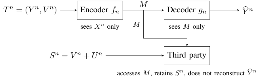
Fig. 1. The system. The encoder observes the source X^n alone and stores the description M at rate R_n ; the decoder reconstructs from M alone; the third party retains the side information S^n and accesses the stored index M in order to erase it; it never reconstructs. The figure shows the Gaussian instantiation, where the encoder observes T = (Y, V) , S = V + U with U independent of T , and the reproduction is \hat{Y}^n , an estimate of Y^n alone; the general discrete theorem reproduces the full letter.
