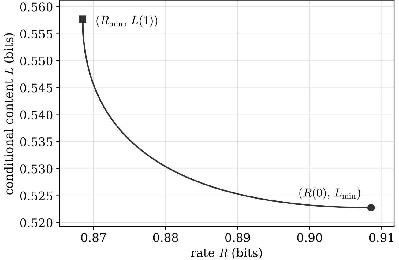
Fig. 2. The Pareto frontier of the rate-content region at (\rho^2, \tau^2, D) = (0.75, 0.5, 0.3) , traced by the two-water-level system of Theorem 12. The tradeoff is strict: the rate-optimal channel pays L(1) - L(D) = 0.0349 bits of excess conditional content, and the content-optimal channel pays R(0) - R_{\min} = 0.0400 bits of excess rate.
