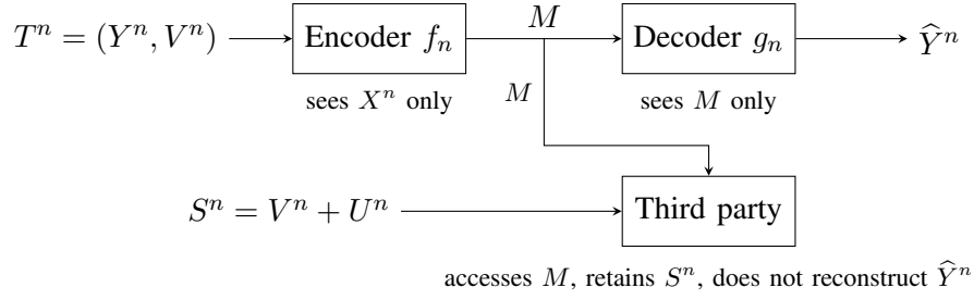
Fig. 1. The system. The encoder observes the source X^n alone and stores the description M at rate R_n ; the decoder reconstructs from M alone; the third party retains the side information S^n and accesses the stored index M in order to erase it; it never reconstructs. The figure shows the Gaussian instantiation, where the encoder observes T = (Y, V) , S = V + U with U independent of T , and the reproduction is \hat{Y}^n , an estimate of Y^n alone; the general discrete theorem reproduces the full letter.
