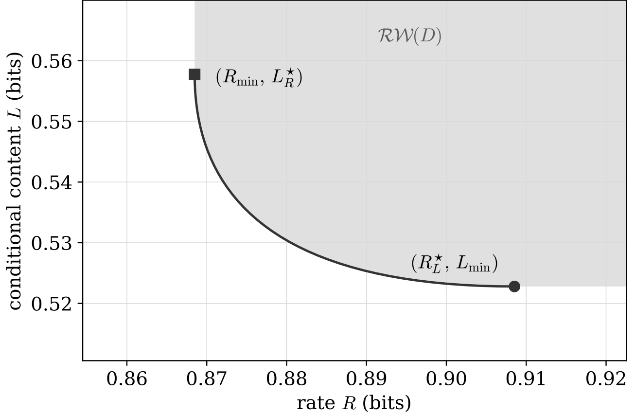
Fig. 2. The rate-content region \mathcal{RW}(D) (shaded) and its Pareto frontier at (\rho^2, \tau^2, D) = (0.75, 0.5, 0.3) , the second instance of Table II at D = 0.3 , traced by the two-noise-fraction system of Theorem 15(b). The tradeoff is strict: the rate-optimal channel pays L_R^*(D) - L(D) = 0.0349 bits of excess conditional content, and the content-optimal channel pays R_L^*(D) - R_{\min} = 0.0400 bits of excess rate.
