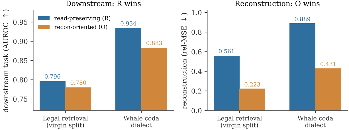
Figure 1: The flip, on two real held-out consumers. At matched bits the read-preserving code (R) beats the reconstruction-oriented code (O) on the downstream task (left; AUROC \uparrow ) while O reconstructs the raw signal better (right; relative MSE \downarrow ). The two fidelities move in opposite directions — a code can win reconstruction and lose the task. Numbers are held-out (legal on the virgin split, §4; whale n=2907 ).
