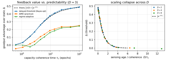
Fig. 8. Controller-level validation of the feedback-usefulness law. Left : goodput advantage over static vs. capacity coherence time \tau_c at D=3 . The Bayes-optimal controller lies on the predicted \frac{1}{2}r(D) (dashed) to within 0.013; practical AIMD falls below static once \tau_c \lesssim D ; the regime-adaptive controller tracks the envelope. Right : sweeping D collapses the optimal advantage onto \frac{1}{2}e^{-D/\tau_c} vs. D/\tau_c .
