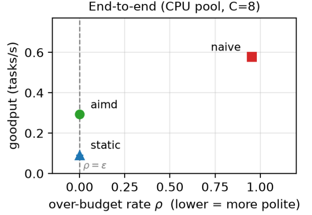
Fig. 5. Goodput vs. over-budget \rho , CPU pool ( C=8 ). With surplus capacity the separation widens: aimd delivers 3.18 \times static's goodput at \rho = 0 , while naive buys goodput only by flagrant over-admission ( \rho = 0.95 ).
