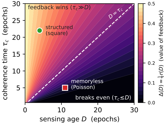
Fig. 3. The impossibility as a map (Cor. 1, 2). The value of feedback \Delta(D) = \frac{1}{2}r(D) = \frac{1}{2}e^{-D/\tau_c} over the sensing-age/coherence-time plane. Closed-loop admission is worth acting on only in the upper-left, where the guest senses the neighbour faster than it changes ( \tau_c \gg D ); as D grows past the ridge D = \tau_c the advantage decays to zero. The two pre-registered contention regimes of §VIII sit on opposite sides: structured (square) load ( \tau_c \gg D ) near the maximum, memoryless (Poisson) load ( \tau_c \lesssim D ) at the floor—the null the regime-adaptive controller is built to detect. Marker placement is illustrative.
