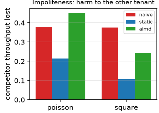
Fig. 5. Harm to the other tenant (throughput lost). naive steals \sim 38\% in both regimes; aimd spares the neighbour under structured contention (24%), but under memoryless contention its mistimed admissions harm it as much as—here more than—naive (45%): the same D -limited failure as its goodput.
