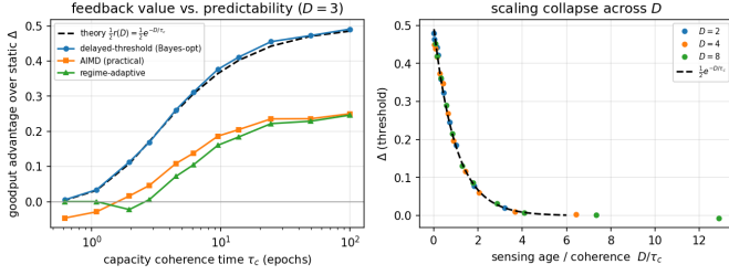
Fig. 6. Controller-level validation of the feedback-usefulness law. Left : goodput advantage over static vs. capacity coherence time \tau_c at D=3 . The Bayes-optimal controller lies on the predicted \frac{1}{2}r(D) (dashed) to within 0.013; practical AIMD falls below static once \tau_c \lesssim D ; the regime-adaptive controller tracks the envelope. Right : sweeping D collapses the optimal advantage onto \frac{1}{2}e^{-D/\tau_c} vs. D/\tau_c .
