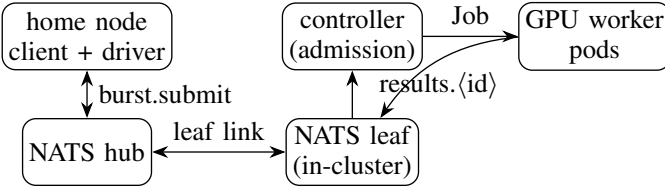
Fig. 1. PoliteBurst architecture. The home client submits over a federated NATS leaf link; the in-cluster controller admits jobs (pacing concurrency to the politeness budget) and launches GPU worker pods, whose results route back through the leaf.
