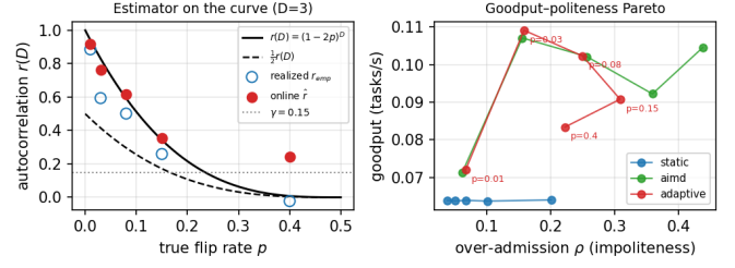
Fig. 7. Live regime-adaptive controller on 2 \times \text{GV100} (Markov \tau_c sweep, D=3 , two seeds). Left : the online estimate \hat{r} and the realized availability autocorrelation r_{\text{emp}} land on (1-2p)^D ; the closed-loop/static switch fires as r(D) crosses \gamma . Right : the goodput-over-admission Pareto—adaptive tracks AIMD when feedback is useful and peels off toward static’s politeness as p grows, shedding over-admission exactly where r(D) \rightarrow 0 .
