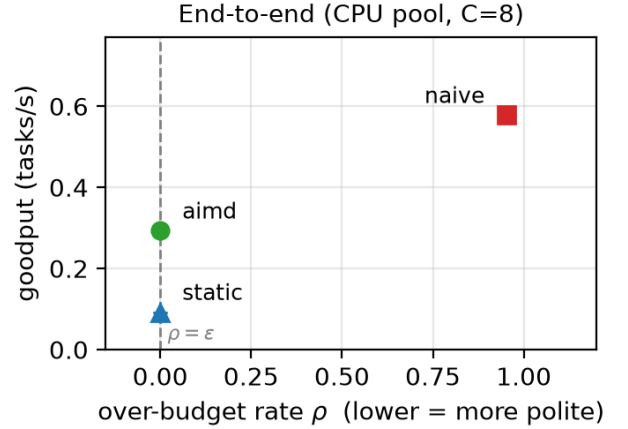
Fig. 3. Goodput vs. over-budget \rho , CPU pool ( C=8 ). With surplus capacity the separation widens: aimd delivers 3.18 \times static's goodput at \rho = 0 , while naive buys goodput only by flagrant over-admission ( \rho = 0.95 ).
