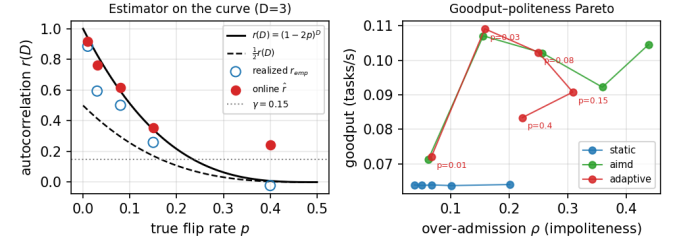
Fig. 8. Live regime-adaptive controller on 2 \times \text{GV100} (Markov \tau_c sweep, D=3 , two seeds). Left : the online estimate \hat{r} and the realized availability autocorrelation r_{\text{emp}} land on (1 - 2p)^D ; the closed-loop/static switch fires as r(D) crosses \gamma . Right : the goodput-over-admission Pareto—adaptive tracks AIMD when feedback is useful and peels off toward static’s politeness as p grows, shedding over-admission exactly where r(D) \rightarrow 0 .
