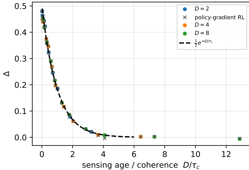
scaling collapse across D
