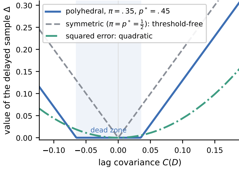
Figure 1: The contact-order trichotomy (Theorem 14), drawn exactly. Polyhedral objective with \pi=.35 , one kink at p^*=.45 , \Delta s=2 : sign-dependent hinges with dead-zone thresholds a^+=.035 (positive branch) and a^-=.065 (negative branch) — anticorrelation of the same magnitude can be worthless where positive correlation has value. The symmetric case is the threshold-free degenerate hinge; squared error responds quadratically with no dead zone. The axis spans exactly the feasible covariance range [-\pi^2, \pi(1-\pi)] ; for stronger asymmetry (e.g. \pi=.2 , p^*=.3 ) the negative-branch threshold exceeds the feasible range entirely and anticorrelated sensing is worthless at every achievable covariance.
