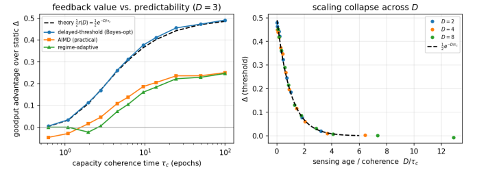
Fig. 8. Controller-level validation of the feedback-usefulness law. Left : goodput advantage over static vs. capacity coherence time \tau_c at D=3 . The Bayes-optimal controller lies on the predicted \frac{1}{2}r(D) (dashed) to within 0.013; practical AIMD falls below static once \tau_c \lesssim D ; the regime-adaptive controller tracks the envelope. Right : sweeping D collapses the optimal advantage onto \frac{1}{2}e^{-D/\tau_c} vs. D/\tau_c .
