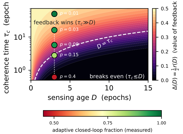
Fig. 2. (a) Under age- D sensing the achievable (\rho, g) pairs form the shaded hull; static policies lie on the diagonal g = \rho , and the closed-loop optimum (\frac{q}{2}, \frac{1-q}{2}) (memoryless threshold m_t = \hat{x}_t ) sits a vertical \Delta(D) = \frac{1}{2}r(D) above it (Thm. 1). (b) The same value \frac{1}{2}e^{-D/\tau_c} over the sensing-age/coherence-time plane (log \tau_c ); points are the measured Markov contention sweep (Cor. 1), each shaded by the adaptive controller’s closed-loop fraction, opening onto static as D crosses \tau_c .
